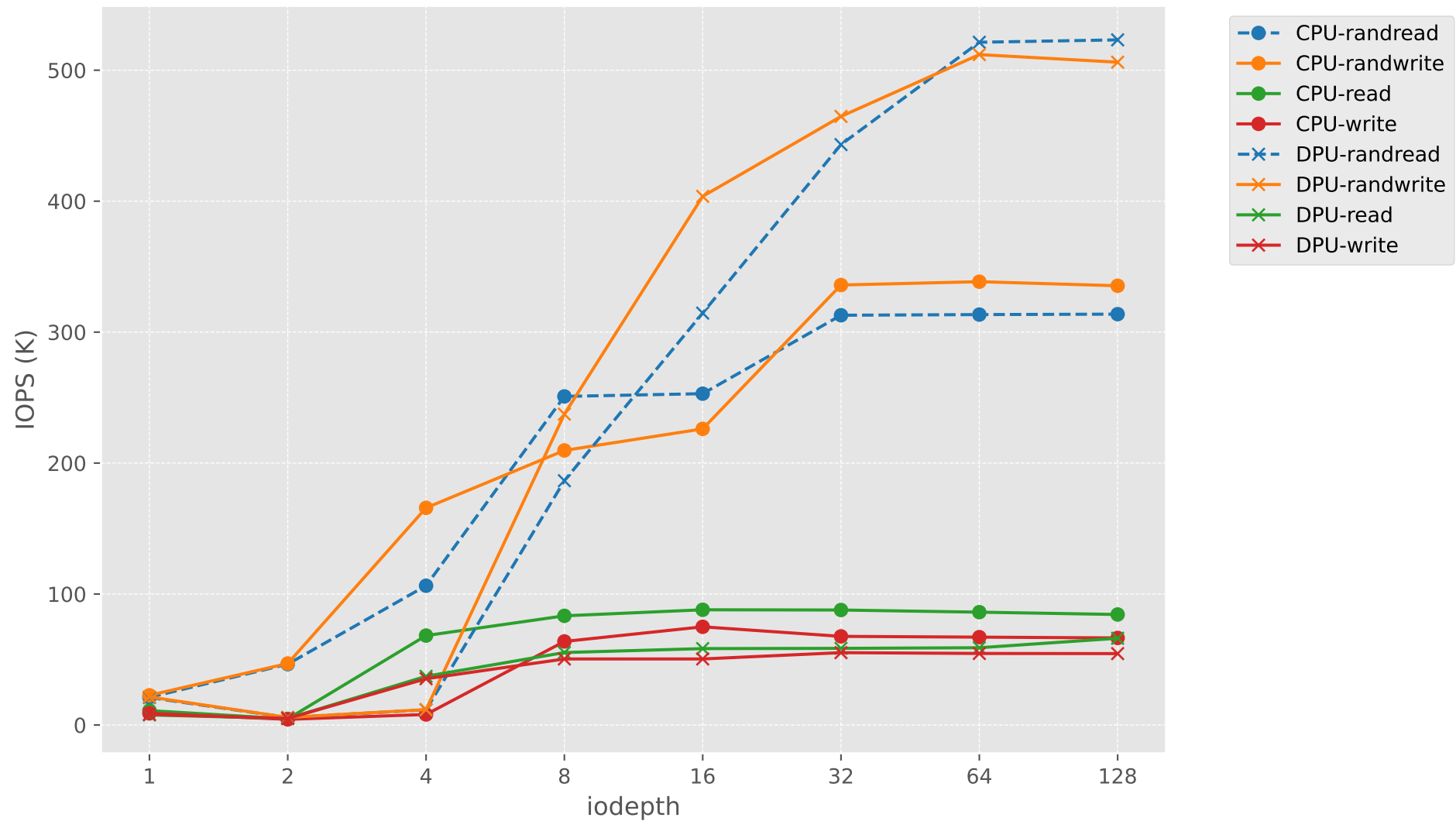
IOPS vs iodepth
